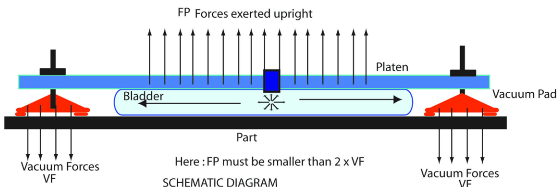
Figure 1: Image of operating principle of OLGA
